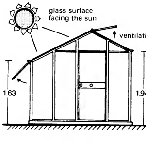
⑦ Solar greenhouse
